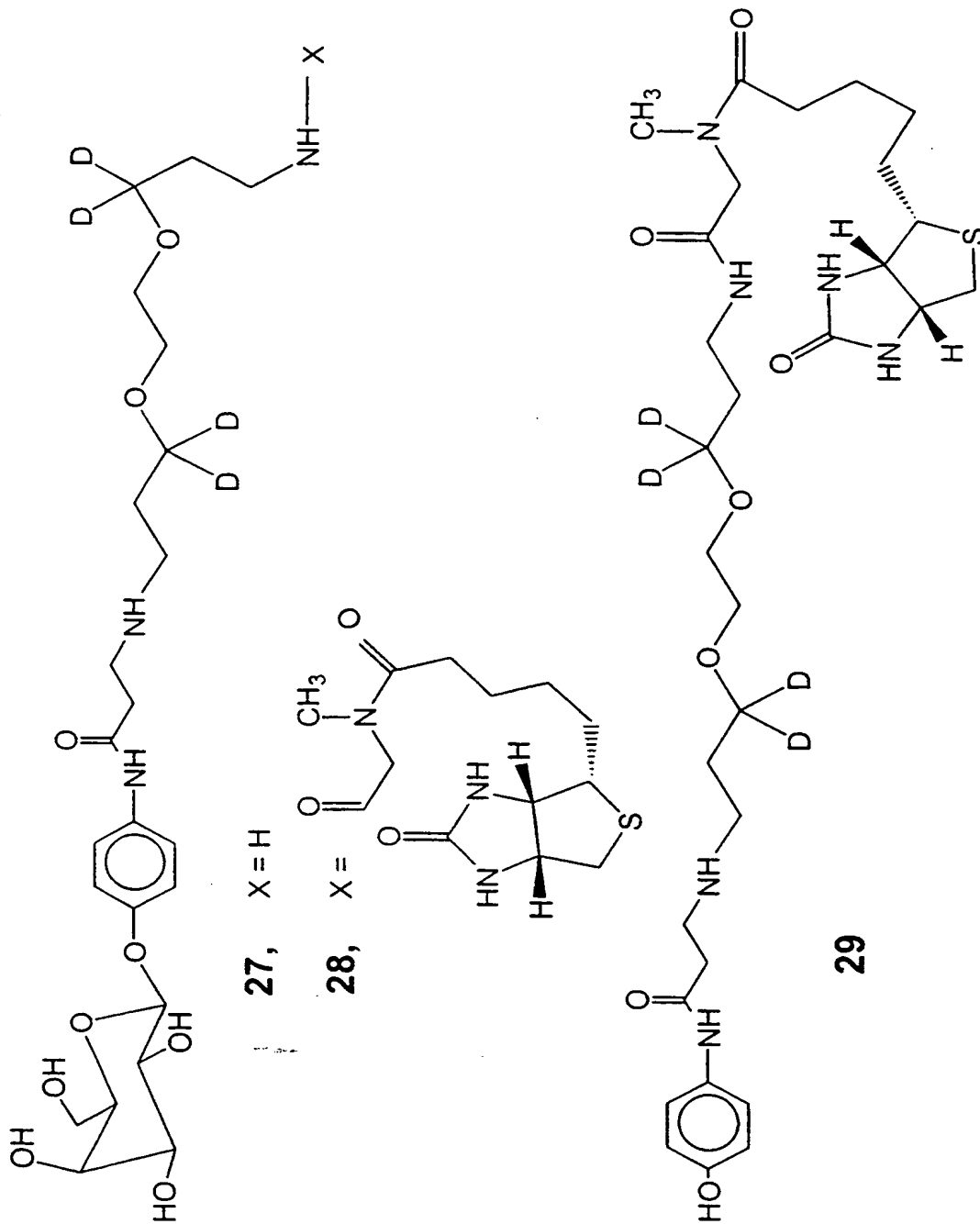
Scheme 19
